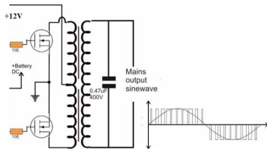
Figure 4: Conversion from Squarewave to Sine wave
