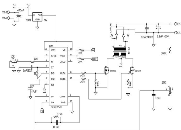
Figure 3: 12V to 220V Inverter Circuit Diagram
