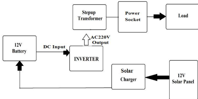
Figure 1: Block Diagram
