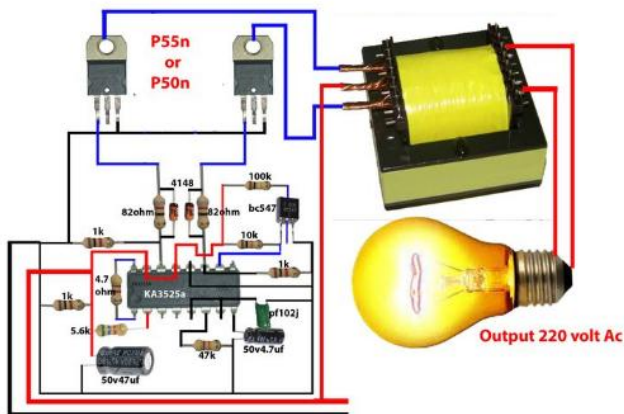
Figure 2: Circuit Diagram
